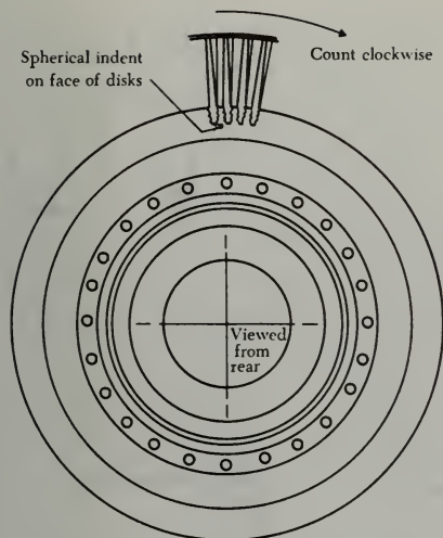
FIGURE 10-63. Turbine blades.
